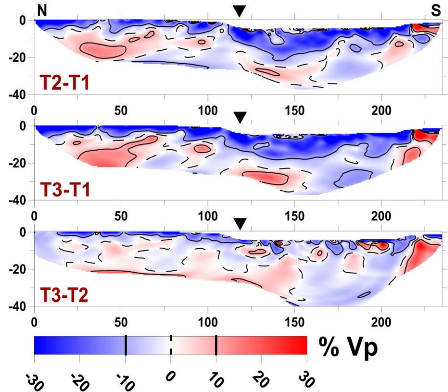
Time-lapse SRT : velocity variations (wet-dry)
