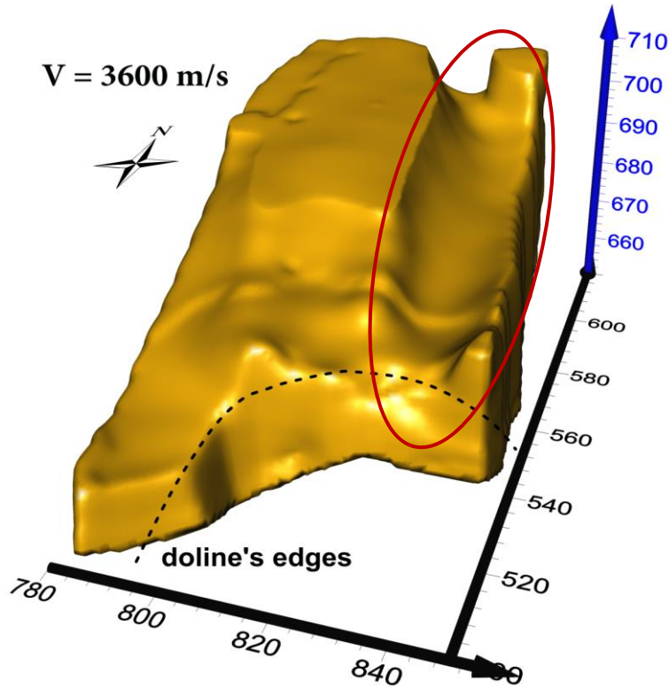
Isosurface of 3D seismic velocity block
